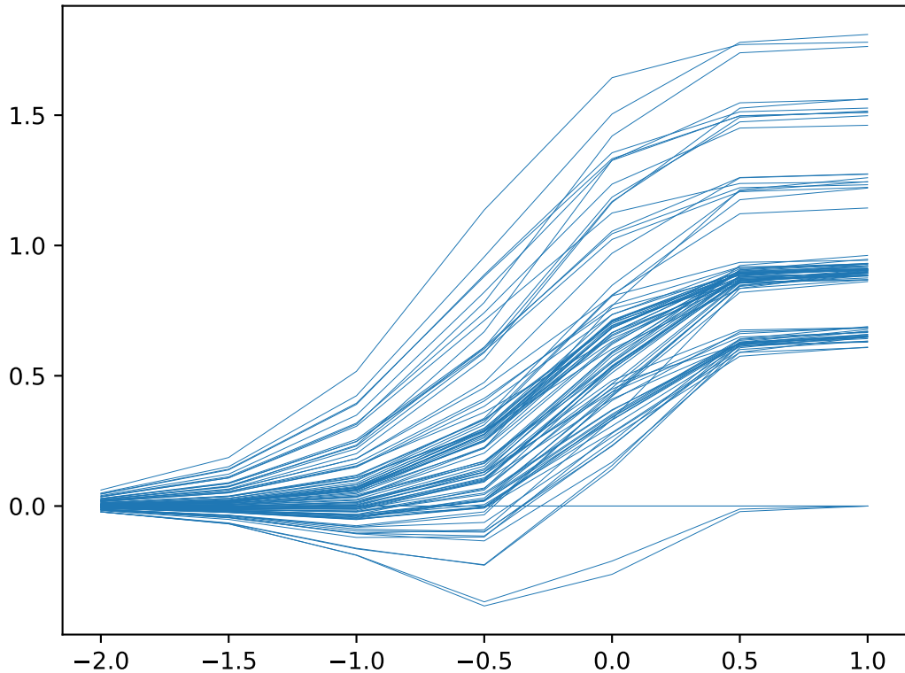
Dynamic Ricci Curvature for Geodesic 0.6000000000000001
